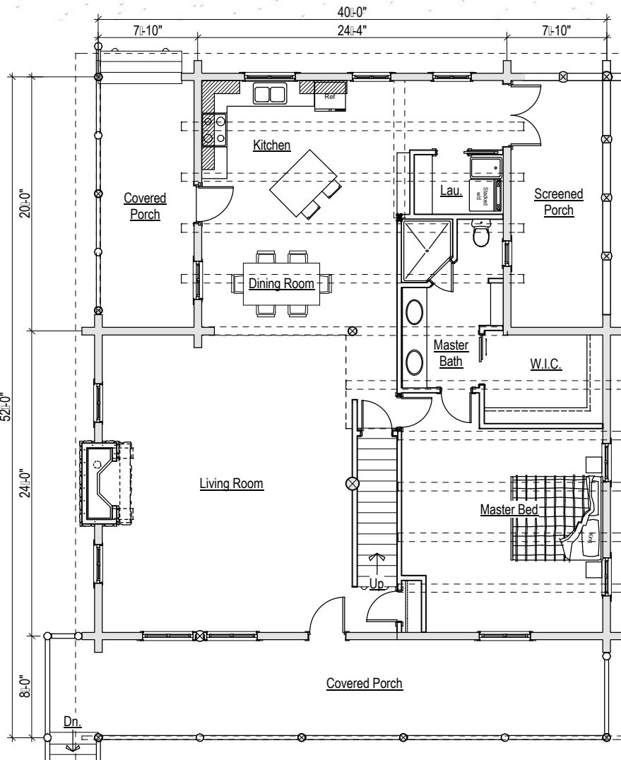
Main Level Plan ○
