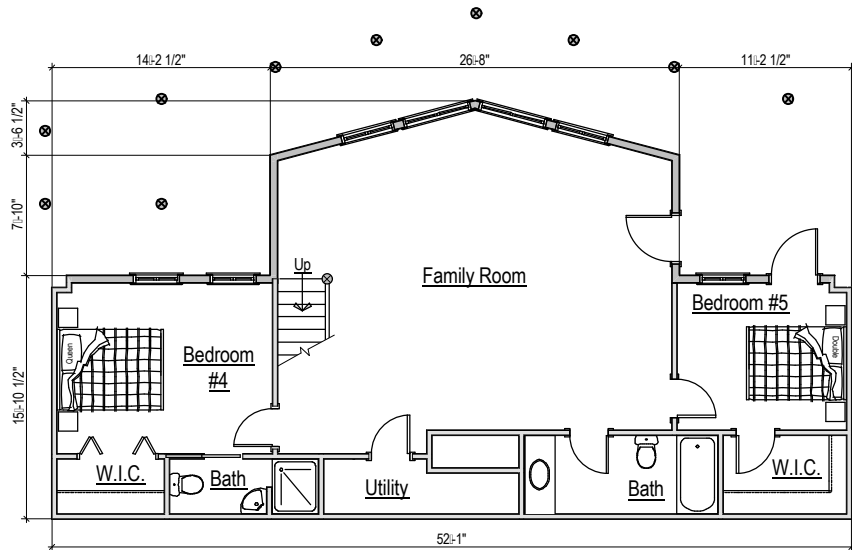
Lower Level Plan ○
