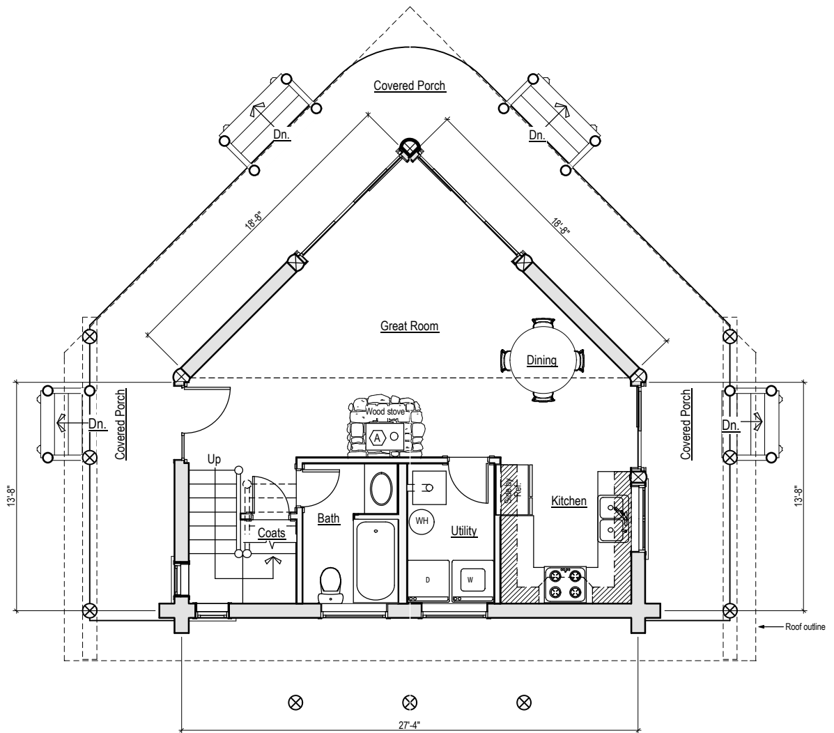
Main Level Plan
