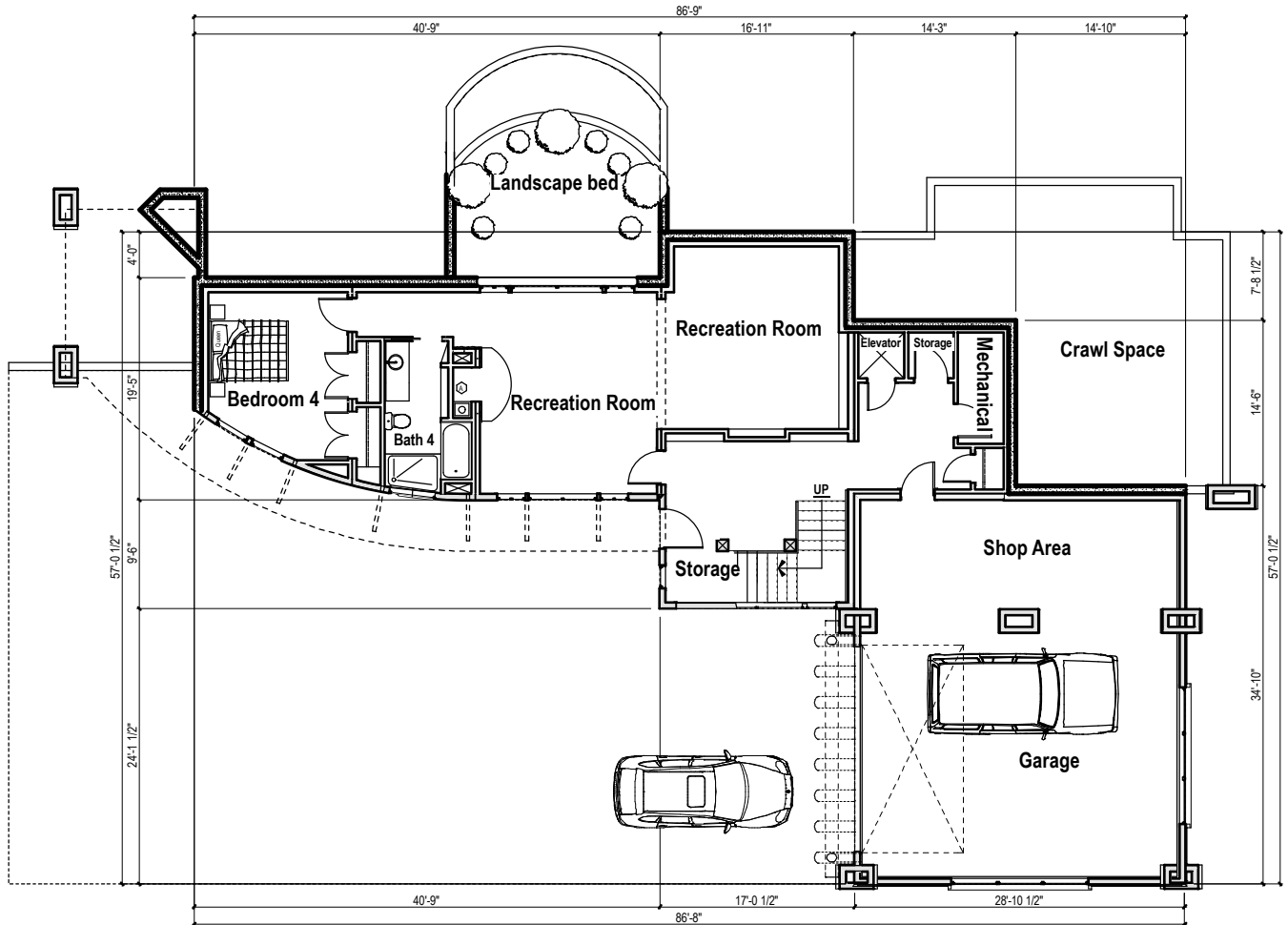
Lower Level Plan
