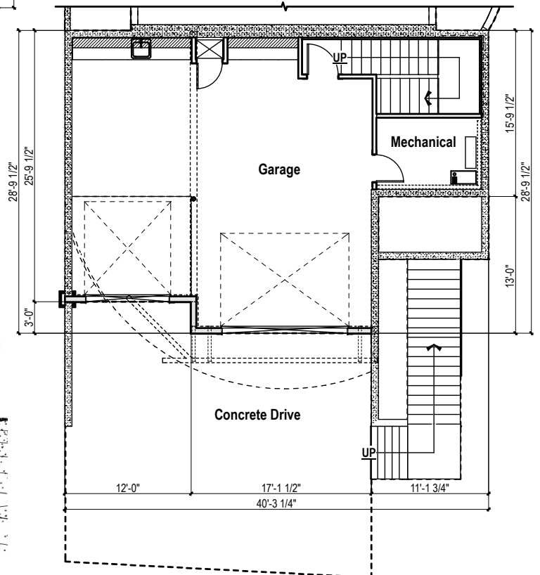
Lower Level
