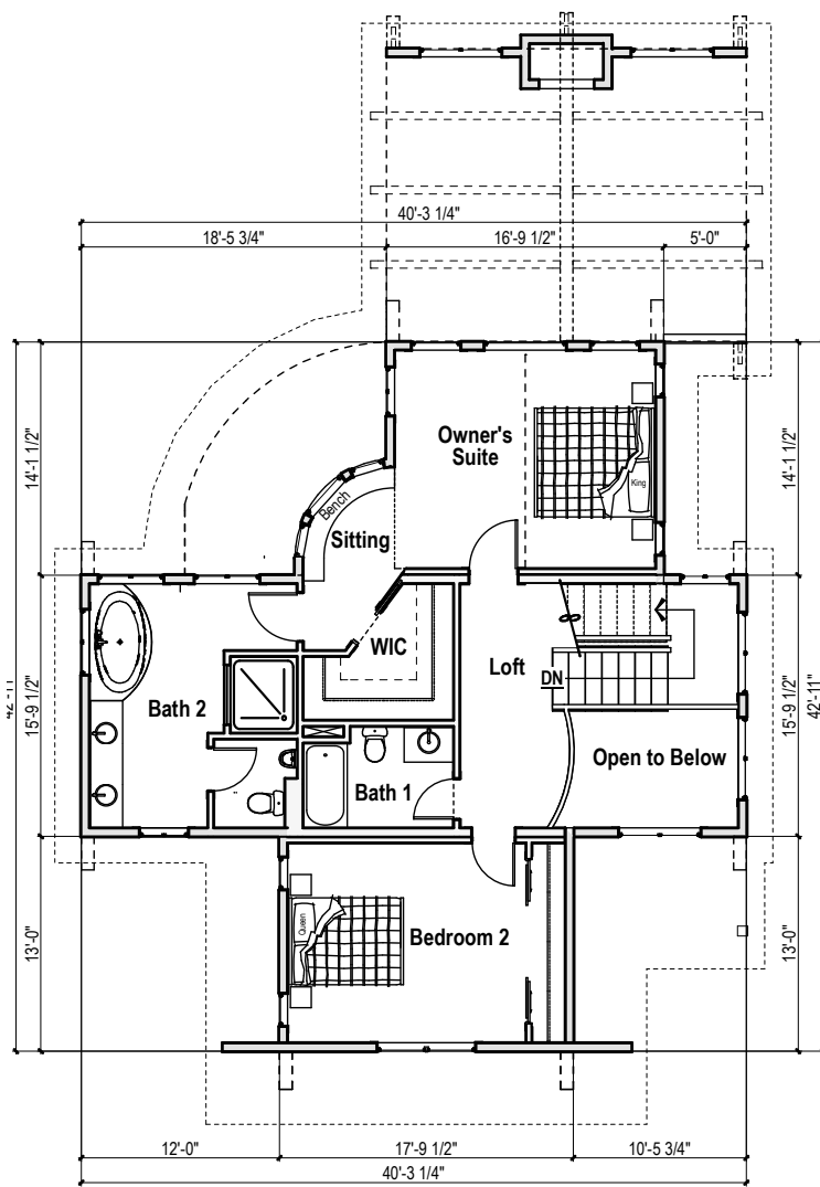
Upper Level
