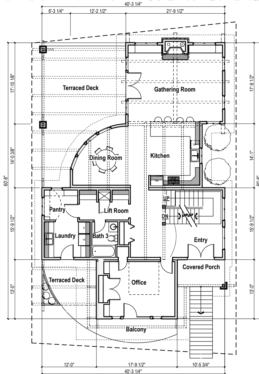
Main Level
